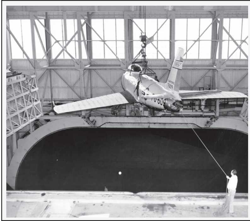
F-86 Airplane Being Lowered Into 40- by 80-foot Wind Tunnel (1954)
